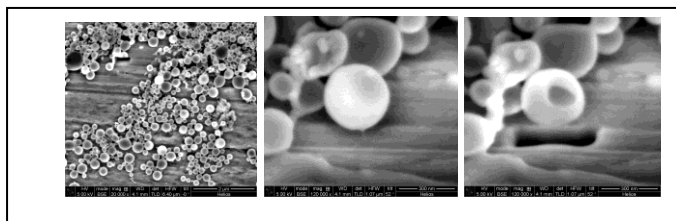
Figure 10. SEM images showing an overview of the HSNS sample (left, scale bar 2 \mu m) and an unetched sphere (middle, scale bar 300 nm), as well as the same sphere after extensive etching with a focused ion beam (right, scale bar 300 nm) [25].
