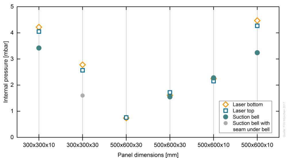
Figure 22: Comparison of the two lift-off measurement techniques. Values from two laser sensors of the vacuum chamber measurements were evaluated by the tangent method
