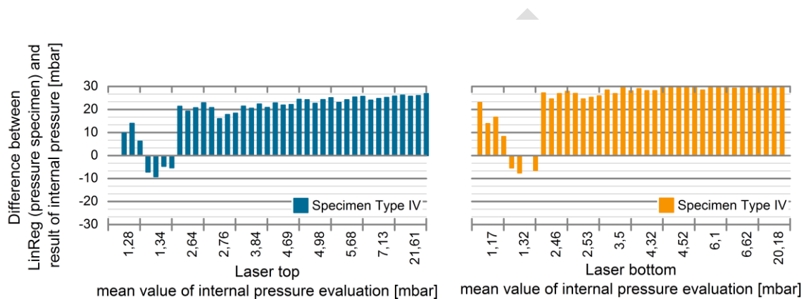
Figure 20: Deviation of the pressure value from linear regression of the internal pressure reading and the result of the evaluation of the internal pressure gained from the foil lift-off measurement for specimen type IV. Data classified to mean values of the internal pressure evaluation to show which four lift-offs belong to one measurement.
