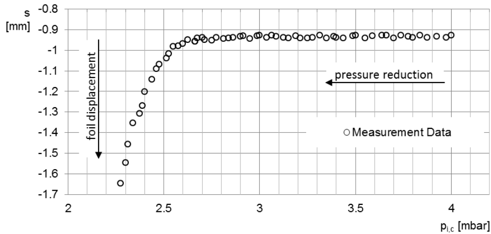
Figure 6: Exemplary measurement data s(p_{i,c}) determined on a VIP with 15 mm thickness, sample rate 1 Hz
