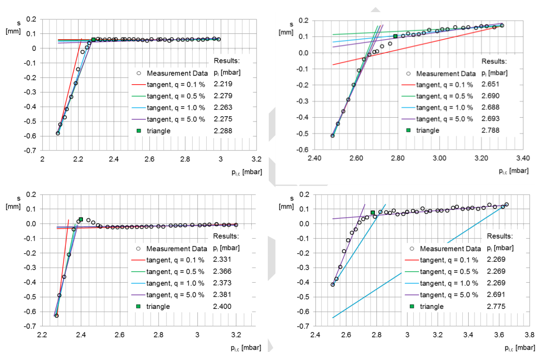
Figure 10: Typical forms of test data including results for the tangent method with different threshold values for q (0.1 %, 0.5 %, 1.0 %, 5.0 %) and the triangle method. Top left: straight flanks and a sharp kink in the bent transition zone; top right: straight flanks and a round bent transition zone; bottom left: straight flanks and a reciprocal foil behavior before the lift-off; bottom right: higher spreading of individual measurement data points (equal tangents for 0.1 %, 0.5 % and 1.0 %)
