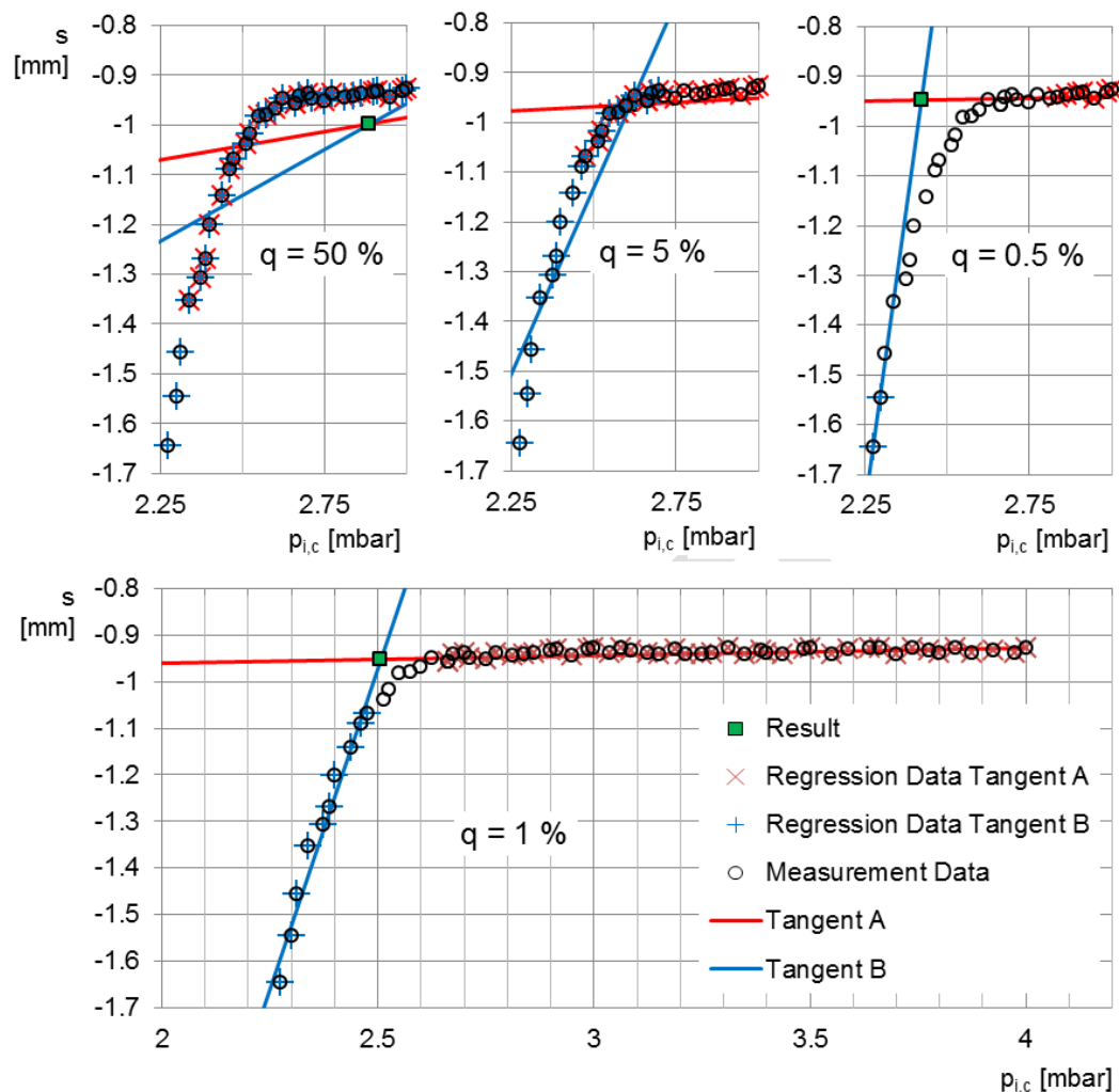
Figure 7: Utilization of the tangent method on exemplary real measurement data; results of analysis with different thresholds of q
