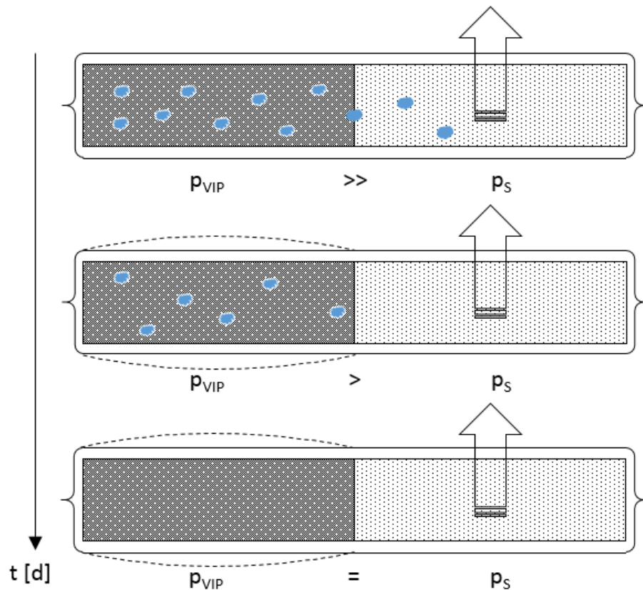
Figure 18: Schematic illustration of the pressure diffusion taking place in the two different types of core material within one specimen. The arrow indicates the position of the leak tight connector where evacuation and internal pressure measurement are conducted.
