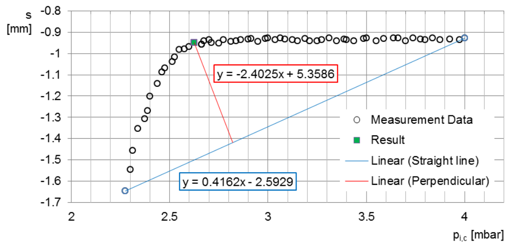
Figure 8: Utilization of the triangle method on exemplary real measurement data
