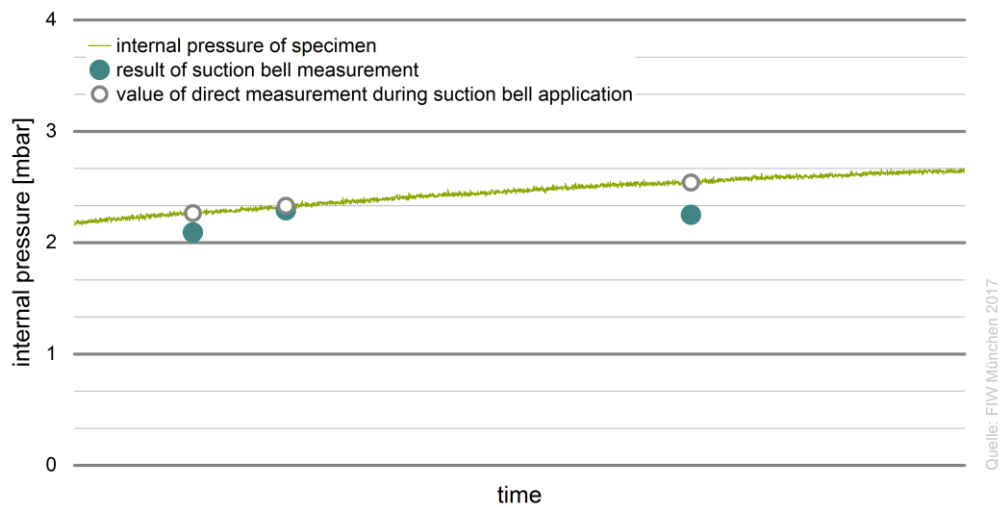
Figure 21: internal pressure behavior during suction bell measurements
